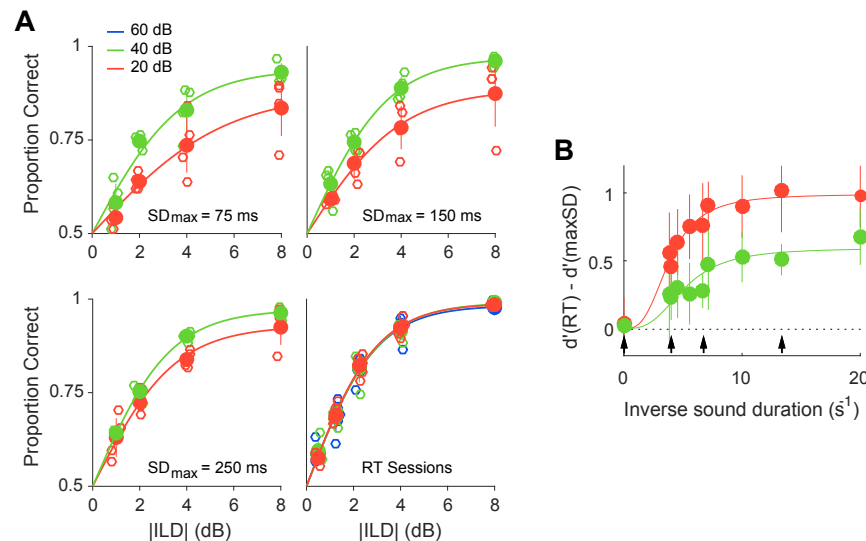
Figure 3: Breakdown of Weber's law for short controlled sound durations (A) Psychometric functions for three conditions where the maximum sound duration SD_{max} was 75, 150, 250 ms and for the RT sessions where the sound always stopped only when the choice was made. Empty dots are individual rats ( n=4 ) and filled dots are mean \pm SD across rats. Fits are from a two parameter logistic function (slope and asymptote; see Methods). (B) Difference between the discriminability index ( d' ) for the RT sessions and for each SD_{max} , separately for each of the two ABLs as a function 1/SD_{max} (filled circles; mean \pm SD across rats). We used 1/SD_{max} to avoid having to arbitrarily specify a SD_{max} for the RT sessions. Lines are fits to a sigmoidal function (see Methods). Arrows show the four SD_{max} for which psychometric functions are shown in (A).
